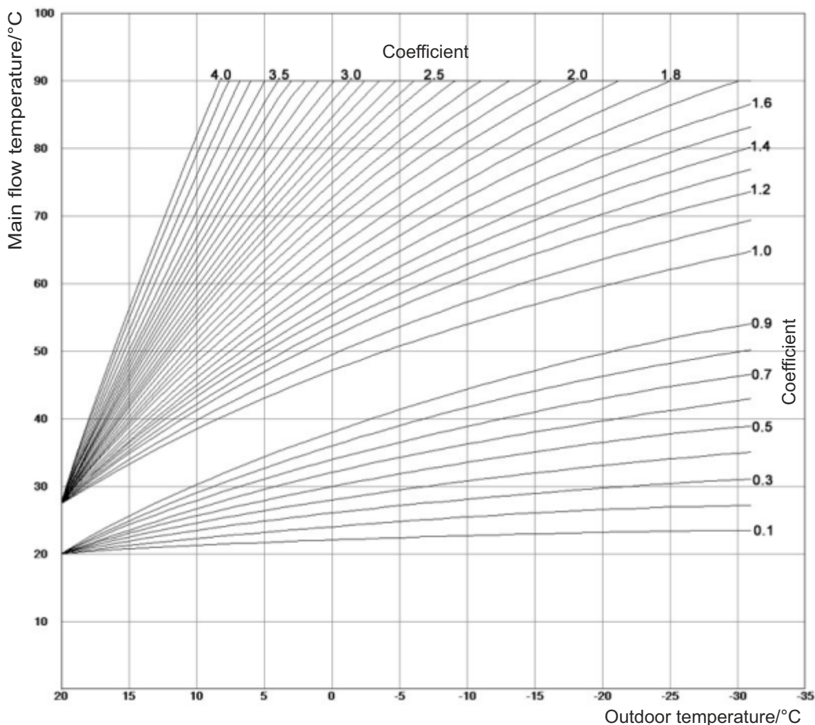
Figure 1: Heating curve
