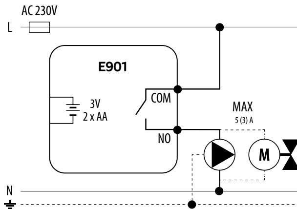
b) Connection diagram to the pump / actuator
