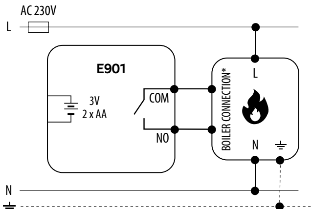
a) Connection diagram to gas boiler
