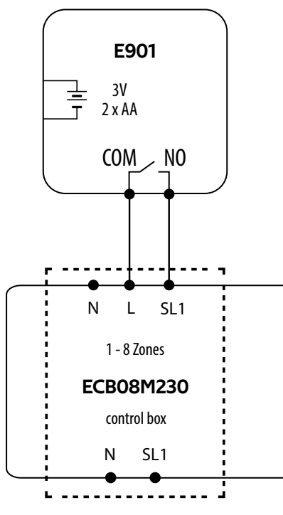
c) Connection diagram to the control box
